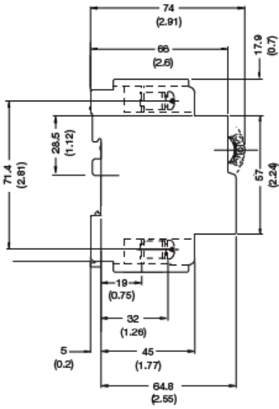
DUAL MOUNT
